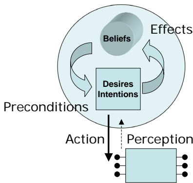
Fig. 2. Agent Architecture
