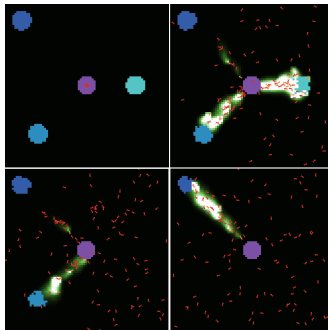
Figure: The snapshots display a simulation of food foraging ants featuring a nest and three food sources. Ants find the shortest path to each source and consume first the closer sources. When no longer reinforced, the pheromone eventually evaporates.
