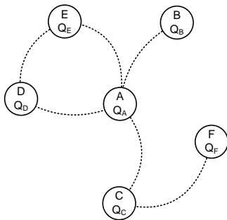
Figure: The reference topology: starting from state A = 36, B = C = D = E = F = 0 the system must evolve into A = B = C = D = E = F = 6 .
