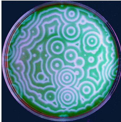
Figure: A snapshot of the Belousov-Zhabotinsky reaction.
