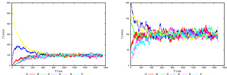
Figure: Two sample simulations from different initial states (left) all items in one node (right) almost sorted
