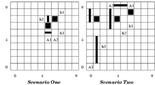
Figure 2: Simulations
