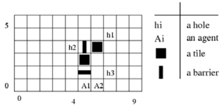
Figure 1: Strongly-Coupled Interactions
