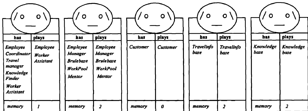
Figure 6: Agent types for the telephone repair service teams case study
