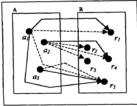
Figure 2: Semantics of role relations
