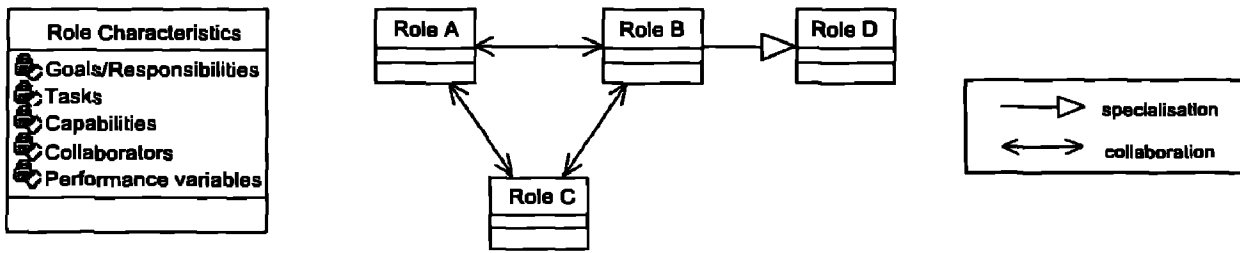
Figure 1: Schematic representation of a role model
