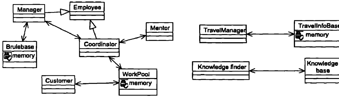
Figure 4: Role models for the telephone repair service teams case study
