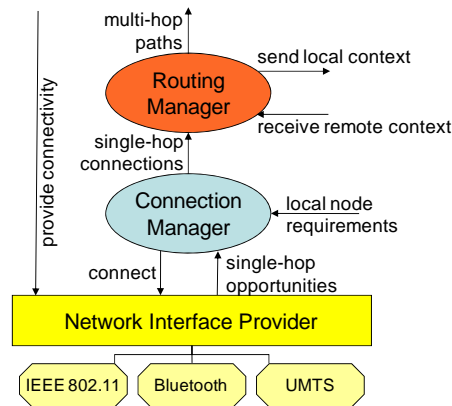
Fig. 2. Our MMHC middleware architecture.
