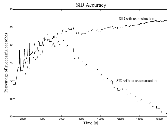
Figure 5. SID accuracy with/without reconstruction in mobile scenarios.
